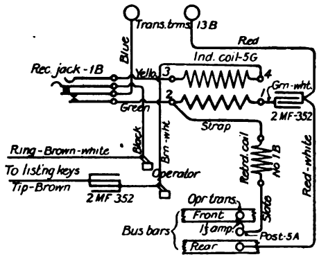
OPERATOR'S TEL. CIRCUIT
